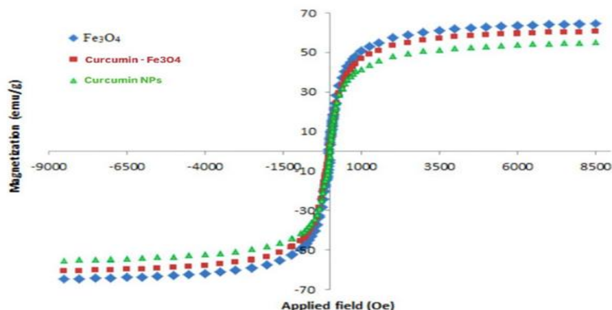
Figure 5. VSM Result,
