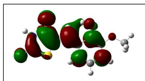
Figure 4: Optimized structure of compound2
