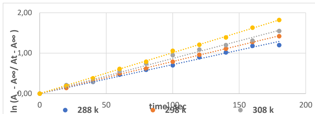
Figure 5. Plot of \ln (A_o - A_\infty / A_t - A_\infty) versus time for hydrolysis of compound A3 at pH = 7 and Temperatures (298, 308, 318, 328°K)
