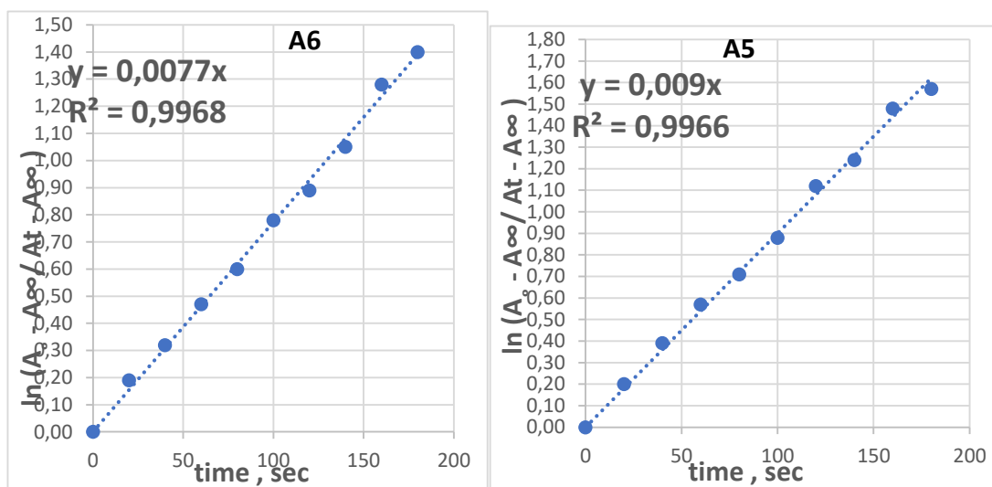
Figure 3. Plot of \ln (A_o - A_\infty / A_t - A_\infty) versus time for hydrolysis of compounds (A5 and A6) at pH = 7 and Temp. 298 °K
