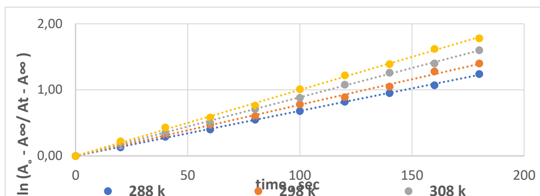
Figure 7. Plot of \ln (A_o - A_\infty / A_t - A_\infty) versus time for hydrolysis of compound A6 at pH = 7 and Temperatures (298, 308, 318, 328°K)
