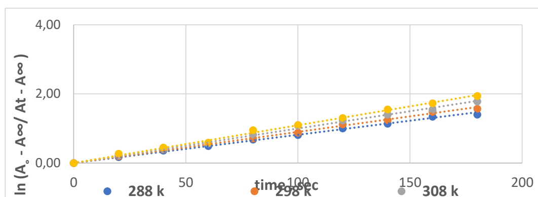
Figure 6. Plot of \ln (A_o - A_\infty / A_t - A_\infty) versus time for hydrolysis of compound A5 at pH = 7 and Temperatures (298, 308, 318, 328°K)
