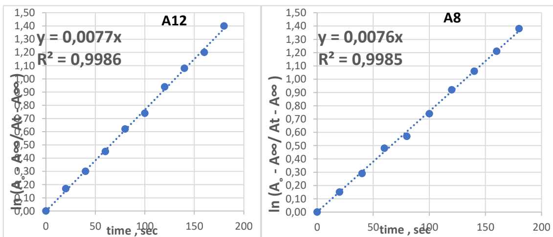
Figure 3. Plot of \ln (A_o - A_\infty / A_t - A_\infty) versus time for hydrolysis of compounds (A8 and A12) at pH = 7 and Temp. 298 °K
